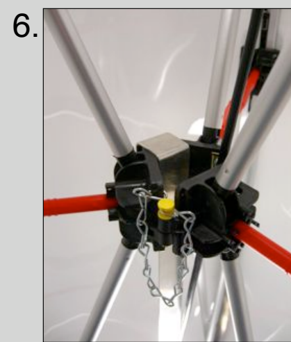
6. Insert the yellow pin that is attached to the jack chain into the hole. There is a total of 4 pins throughout the tower.
