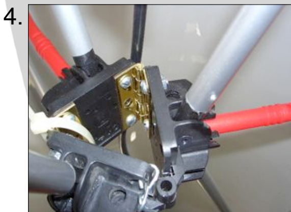
4. Each tower has an opening on the hubs that allows the tower to pop in and out for assemble and packing.
