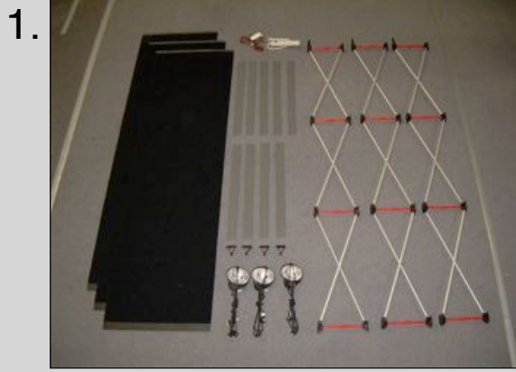
1. All parts above are the parts required to make the PRS 18 tower. There is the popup tower, 9 channel bars, 3 panels, and lights. All of this parts are all part of the tower.
