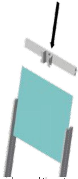
Slide the plexiglass and the octanorm with the monitor bracket attach in between the octanorm uprights. Once the octanorm is goes into the plexiglass lock in place using the tools provided.
